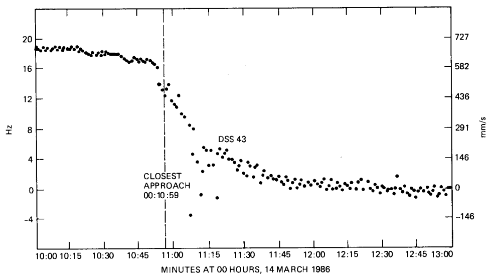
Fig. 7. DSN Giotto encounter one-way Doppler residuals, 1-second count time
