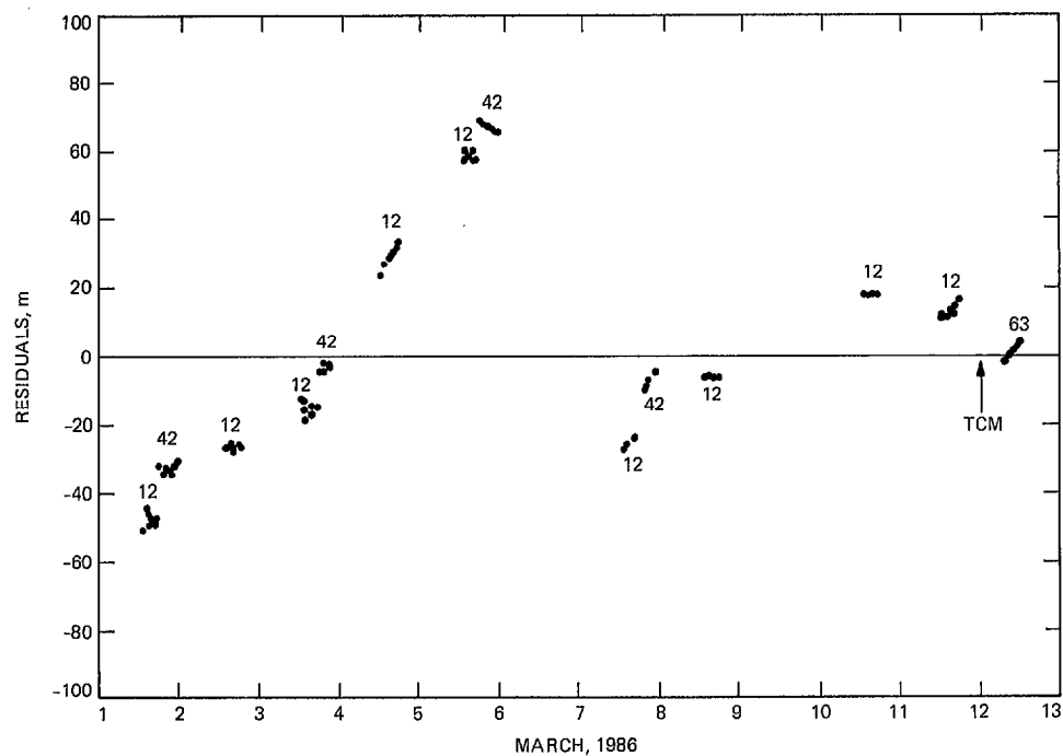
Fig. 4. JPL DSN range residuals from Campaign #2
