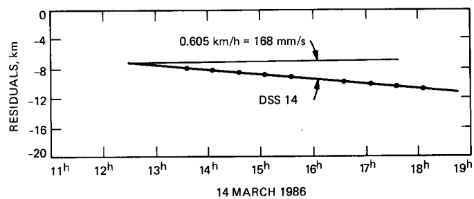
Fig. 6. Post encounter velocity change inferred from range residuals
