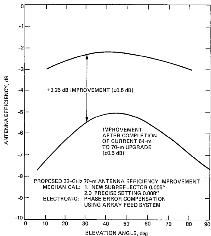
Fig. 4. 70-m antenna performance estimates, "electronic/mechanical" upgrade
