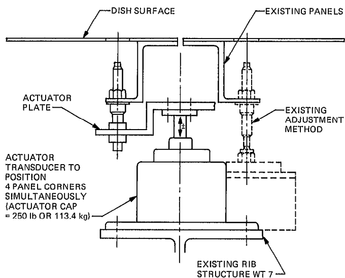
Fig. 3. Reflector panel adjustment, motorized actuator
