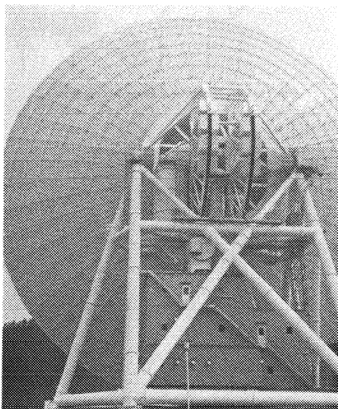
Fig. 6. Usuda 64-m antenna rear view
