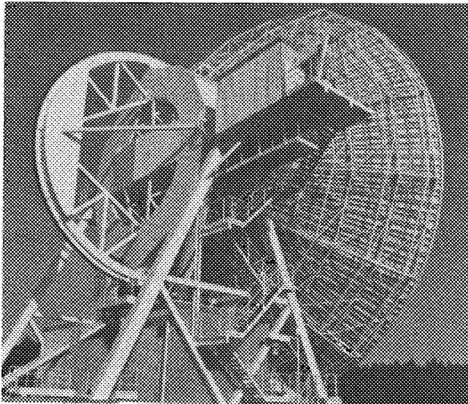
Fig. 2. Weilheim 30-m antenna viewed from rear
