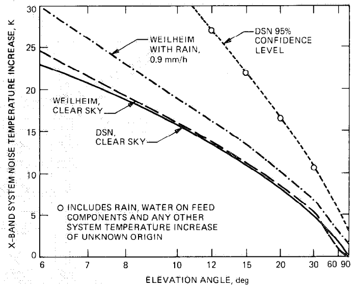
Fig. 14. X-band system temperature increase versus elevation angle
