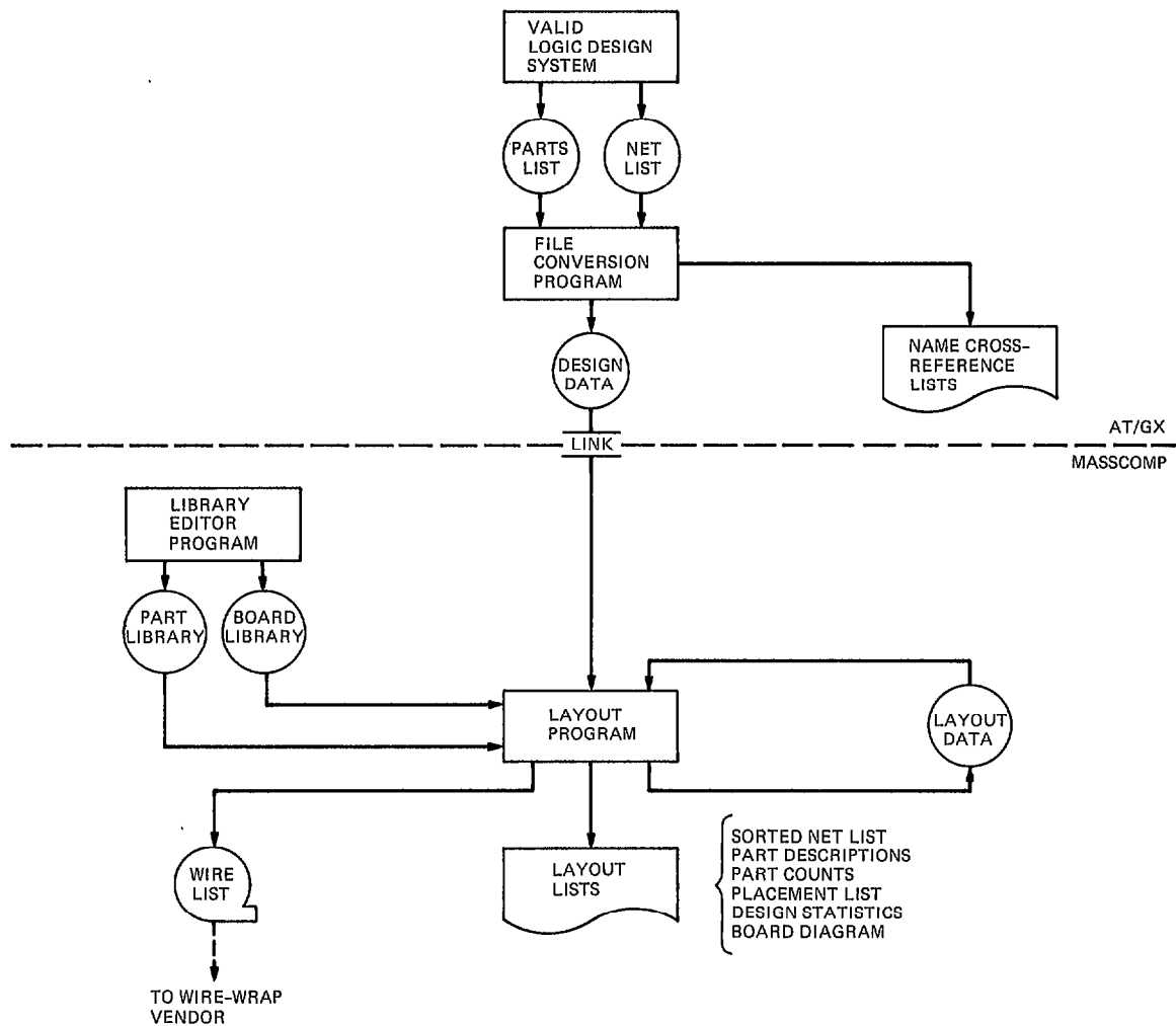
Fig. 1. Layout system
