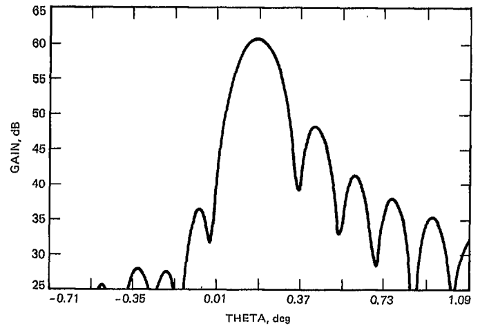
Fig. 3. L-band pattern, present L-band feed location
