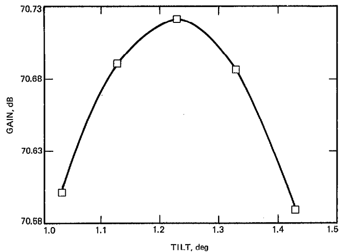
Fig. 12. Gain vs. subreflector tilt (C-band)
