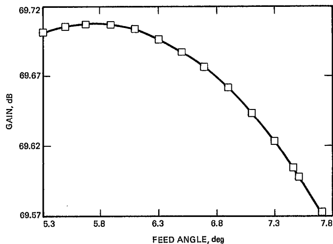
Fig. 9. Gain vs. feed angle (C-band)
