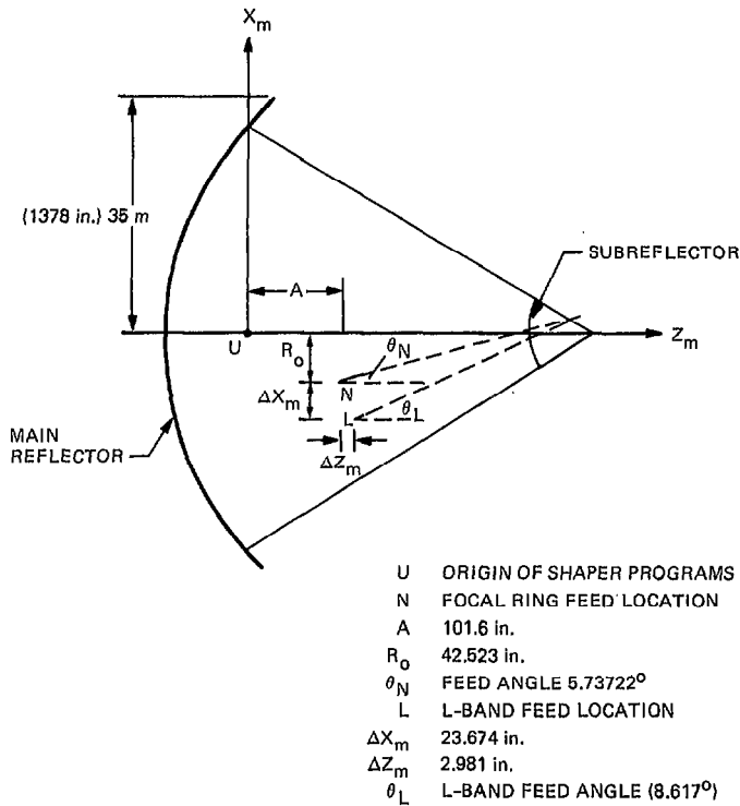
Fig. 1. 70-m antenna geometry
