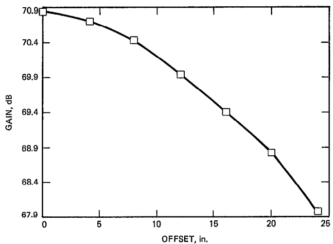
Fig. 6. Gain vs. radial feed displacement (C-band)
