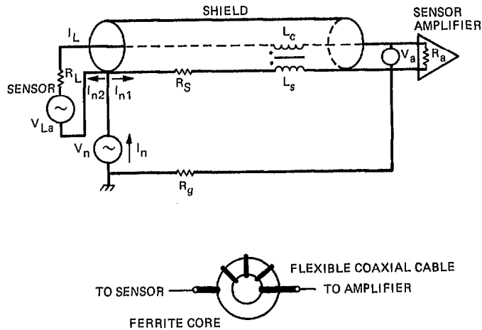
Fig. 1. Coaxial balun placed at the amplifier input
