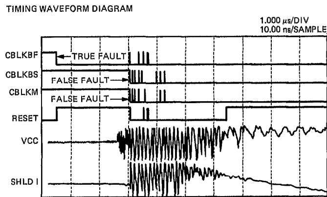
Fig. 2. Crowbar cabinet and instrumentation system noise measurements before improvements
