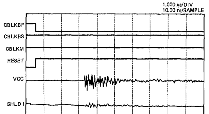
Fig. 3. Crowbar cabinet and instrumentation system noise measurement after improvements
