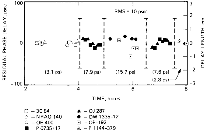
Fig. 3. Phase delay residuals for clusters of 2-3 angularly close radio sources on the DSS 12-DSS 13 baseline. Each source is indicated by a distinct symbol. The vertical dashed lines delimit series of repeated observations for each cluster, and have a height equal to the delay ambiguity at the 8.4-GHz observation frequency. Separate clock offsets were estimated for each series. The RMS scatter for each series is indicated, ranging from 2.8-15.7 psec. The total RMS for all observations is 10 psec.
