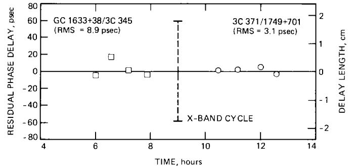
Fig. 4. Differential phase delay residuals for repeated observations of two close quasar pairs, on the 253-km baseline between DSS 13 and the OVRO 40-m antenna. As described in the text, linear combinations are formed for A-B-A observation sequences of each quasar pair to eliminate any linear clock behavior. The total RMS scatter for all eight differential measurements (formed from 24 single source measurements) is 6.7 psec.
