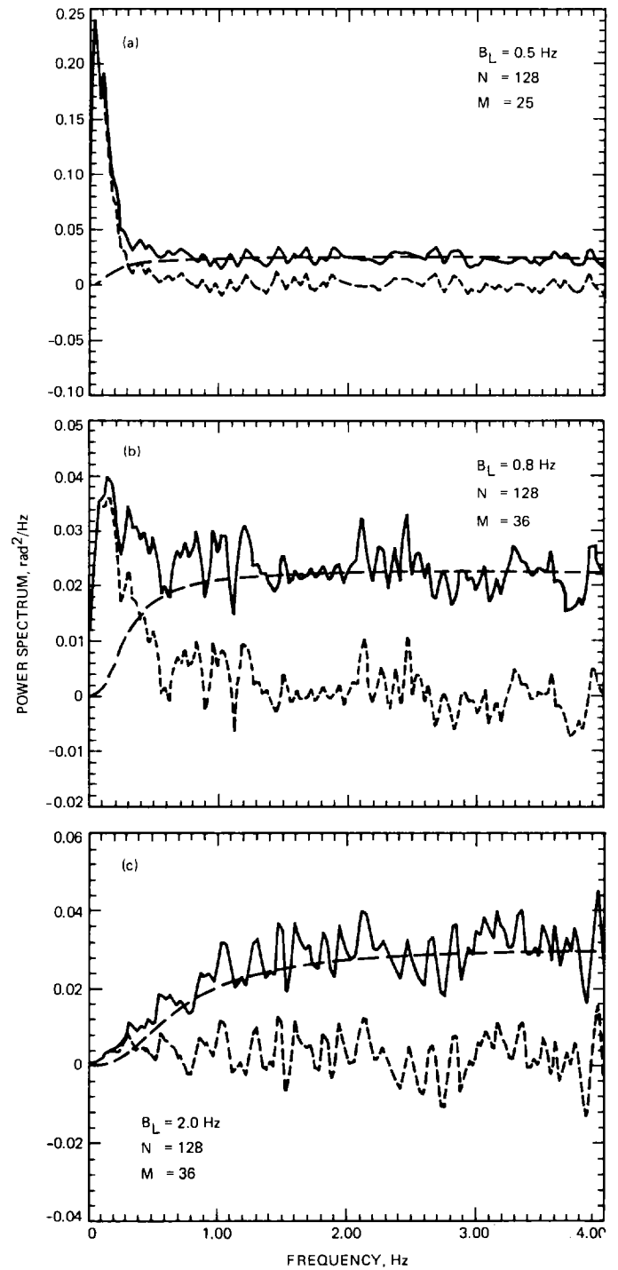
Fig. 6. Spectral density estimates (one-way mode)
