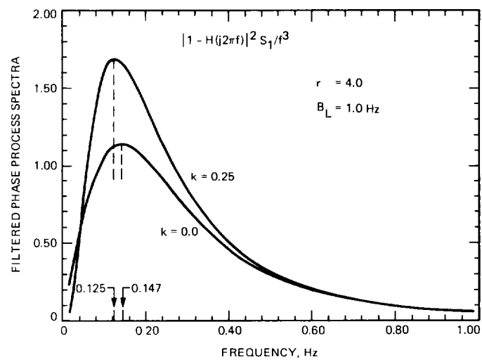
Fig. A1. Filtered process spectra for second and third order loops
