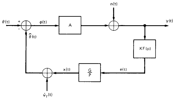
Fig. 1. Receiver phase locked loop block diagram
