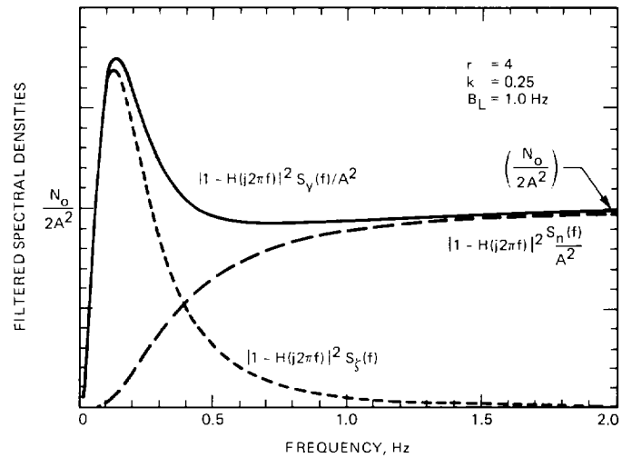
Fig. 4. Filtered spectral densities for a third order loop (inverse f^3 phase process and additive white noise)
