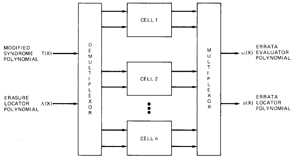
Fig. 4. The new architecture for performing the modified form of Euclid's algorithm
