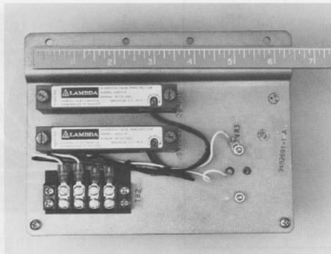
Fig. 8. Overvoltage protection subassembly
