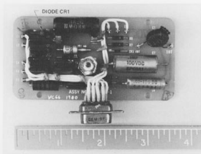
Fig. 3. Modulator and protective circuit printed wiring assembly with burned-out diode CR1 (rating: 45 \pm 1 percent)
