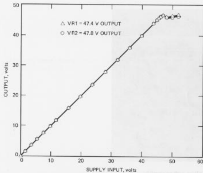
Fig. 5. Clamping voltage test data for modulator and protective circuit subassembly zener diodes VR1 and VR2
