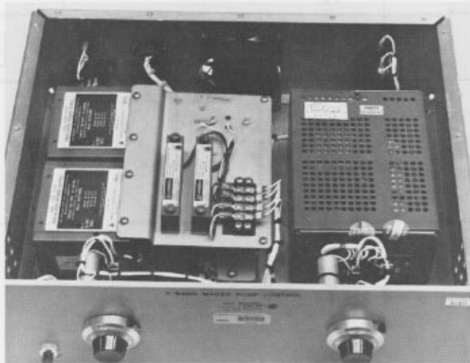
Fig. 7. Pump control with overvoltage protection subassembly installed
