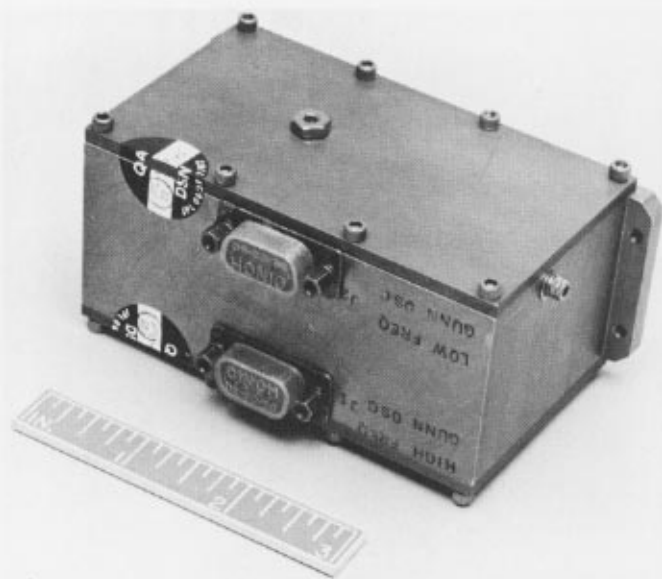
Fig. 2. Modulator and protective circuit subassembly
