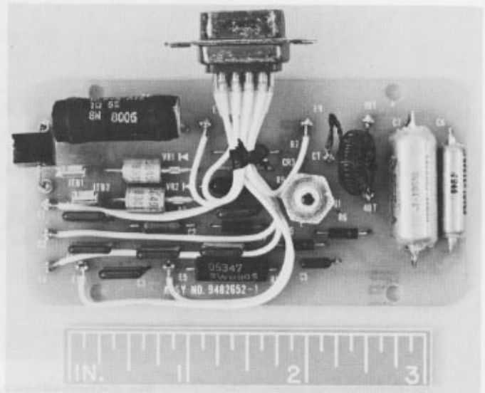
Fig. 6. Modulator and protective circuit printed wiring assembly
