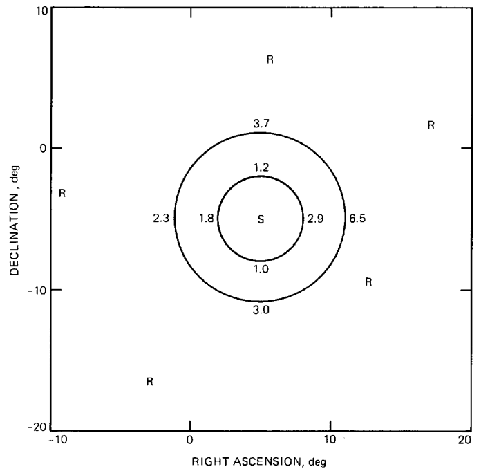
Fig. 4. Differential angular position error due to stationary source structure: the numbers indicate the error, in nanoradians, in a measurement of relative spacecraft position due to time-invariant source structure errors. The numbers apply to a differential position measurement between the S and the indicated point on the circle. All radio sources were assumed to have 5-nanoradian errors in \alpha \cos \delta and in \delta where \alpha is right ascension and \delta is declination.
