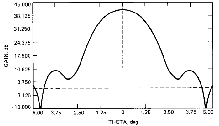
Fig. 8. X-band (8420-MHz) downlink: theta versus gain
