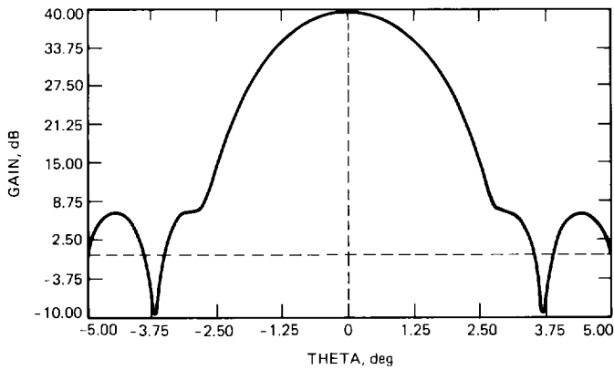
Fig. 7. X-band (7190-MHz) uplink: theta versus gain
