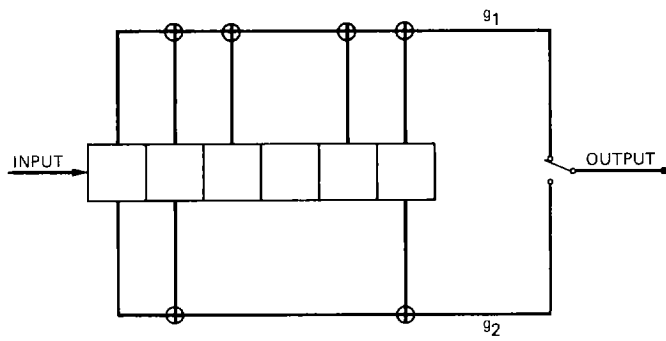
Fig. 2. The K = 6, r = 1/2 encoder
