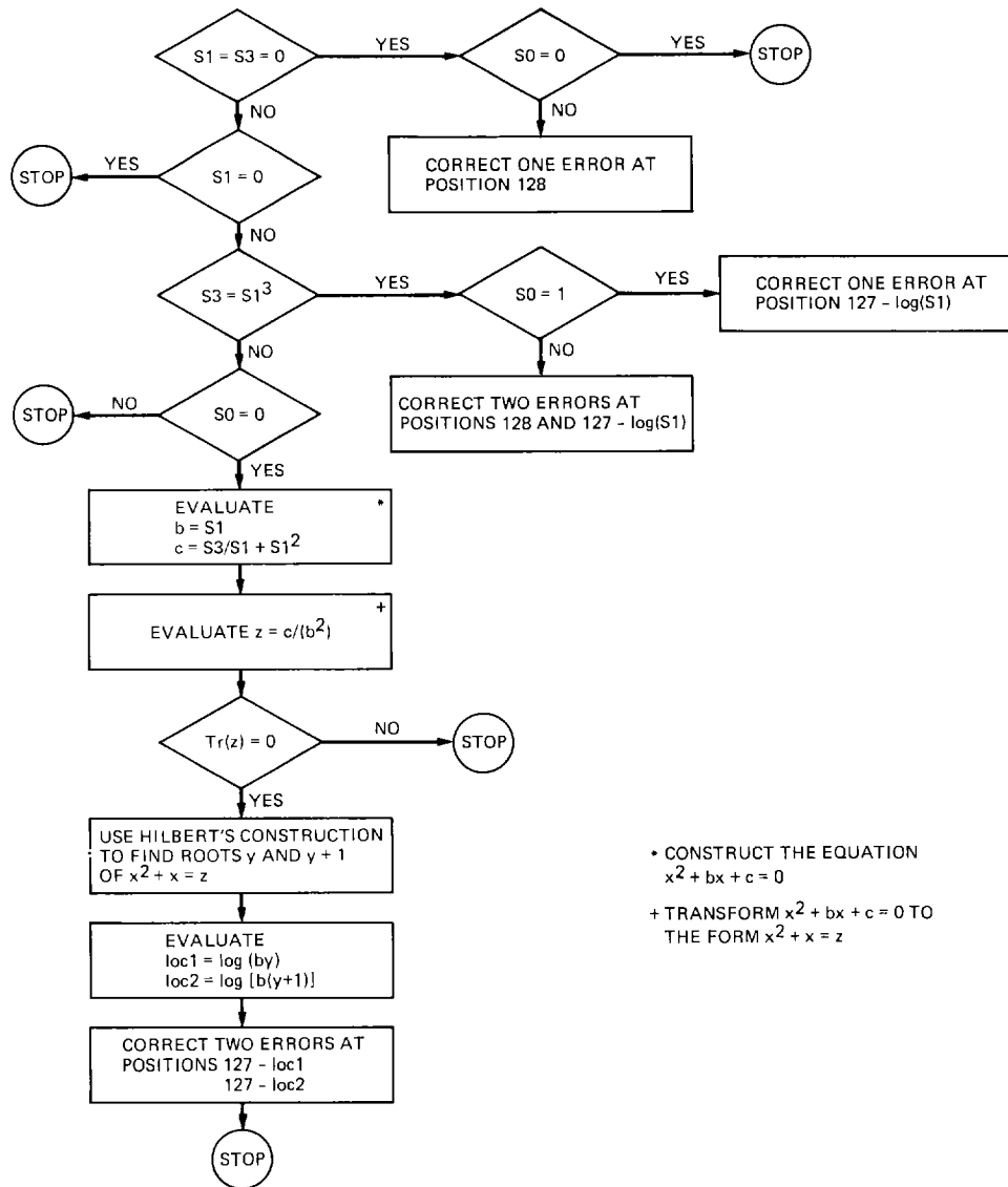
Fig. A-1. Decoding algorithm for the (128,113) BCH code
