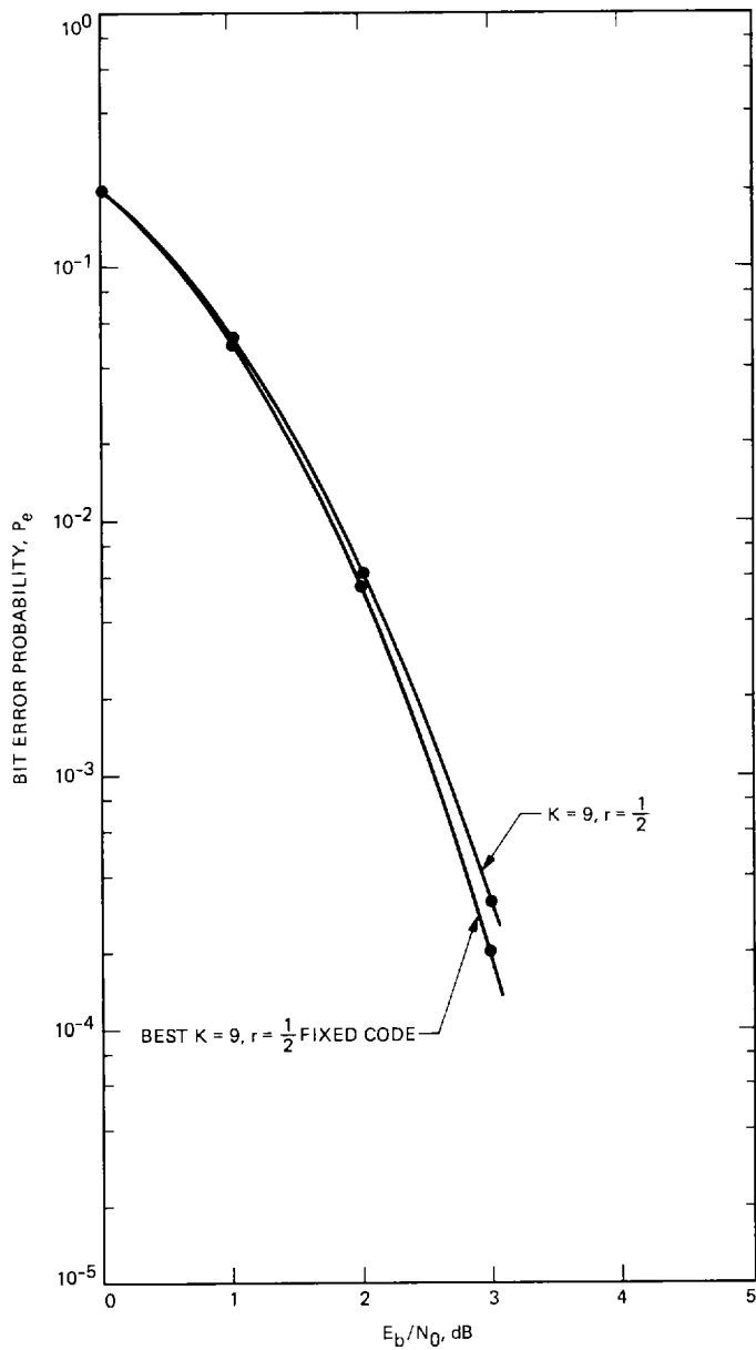
Fig. 5. Performance of two K = 9, r = 1/2 codes
