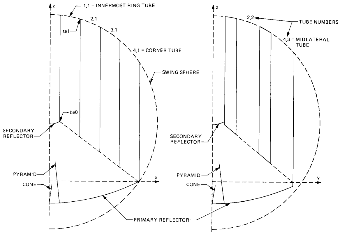
Fig. 6. Cross-sectional views of an integral sunshade on a Cassegrain optical reception antenna within a swing sphere.
