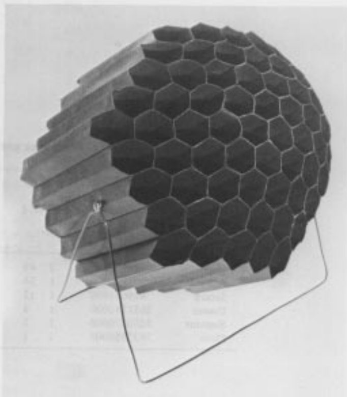
Fig. 3. Overview of a glue-and paper model of an integral sunshade. The telescope looks through the sunshade from behind and below it, in this view. The hexagonal tubes are trimmed to a spherical shape.
