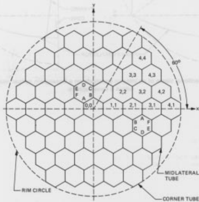
Fig. 5. Plan view of a hexagonally segmented reflector.
