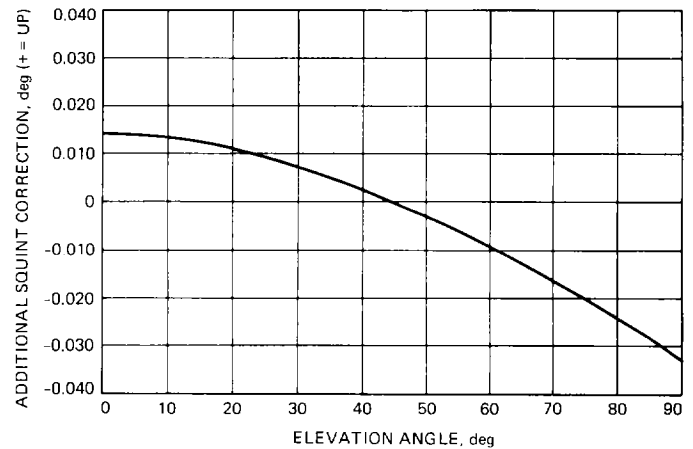
Fig. 8. 70-m antenna additional squint correction needed versus elevation angle.
