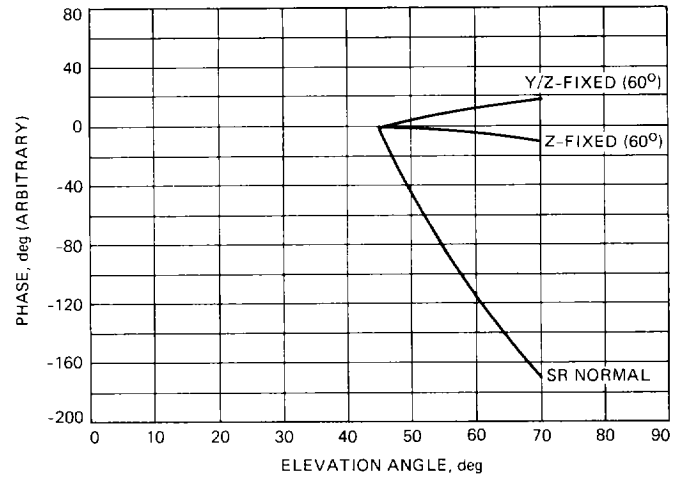
Fig. 4. 70-m antenna GTD-computed phase versus elevation angle, 8420 MHz, for three different subreflector configurations.
