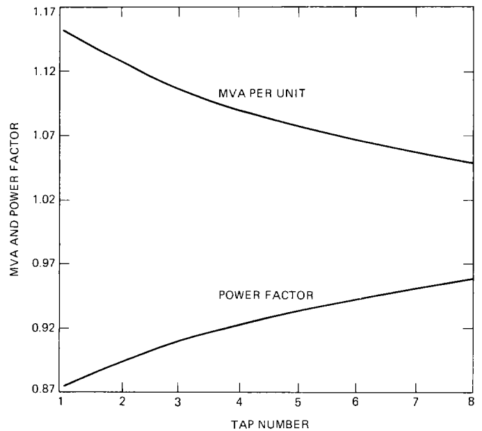
Fig. 9. Generator load.
