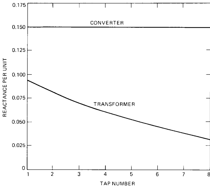
Fig. 8. Load reactance.
