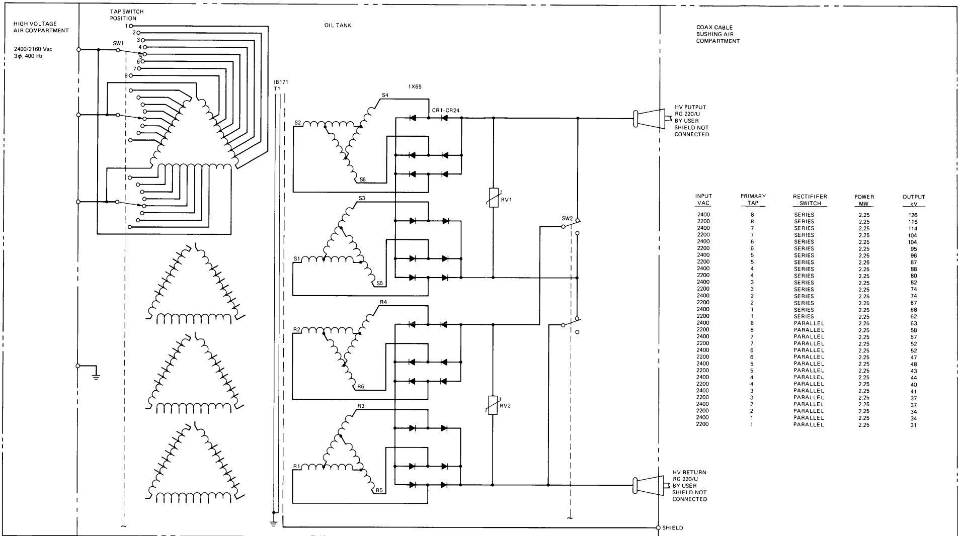
Fig. 2. Transformer rectifier assembly detailed schematic.
