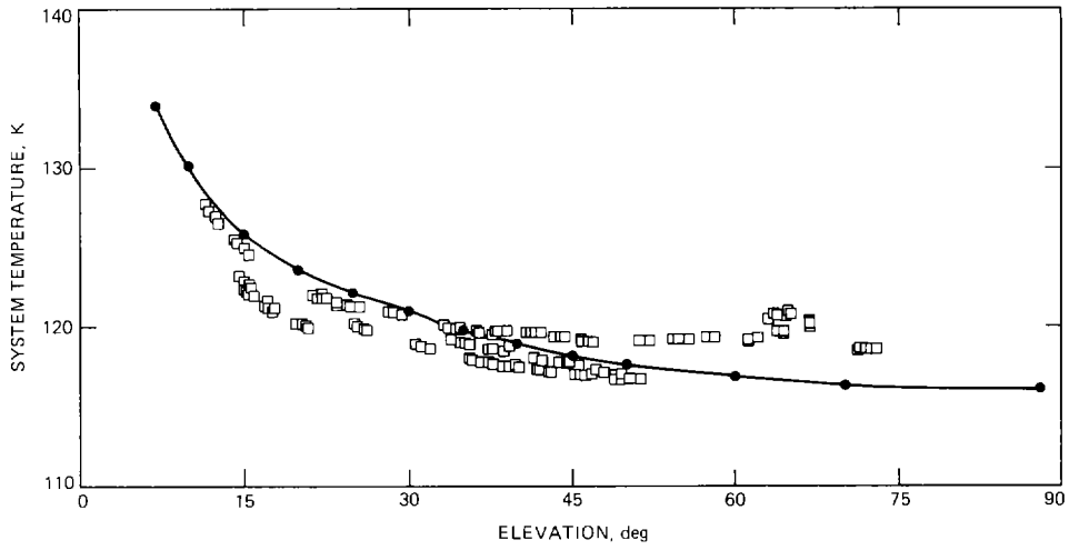
Fig. 2. C-band system temperature.
