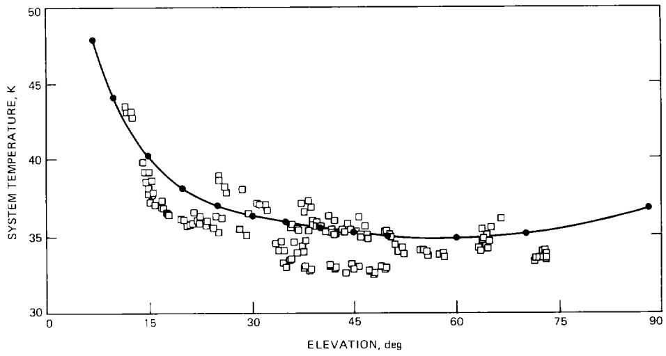
Fig. 3. L-band system temperature.
