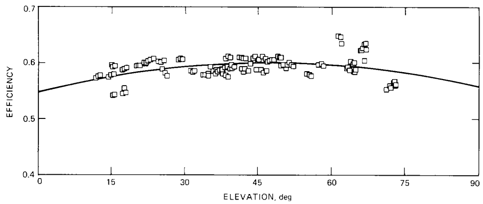
Fig. 5. L-band efficiency versus elevation.
