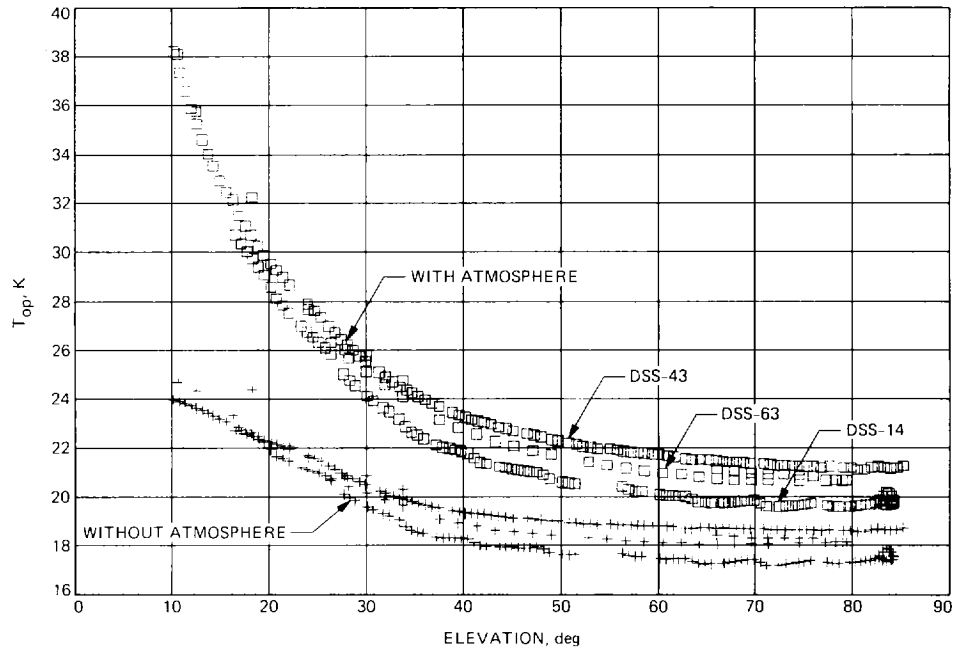
Fig. 1. The 70-m antenna X-band noise temperatures, with and without atmospheric contribution.
