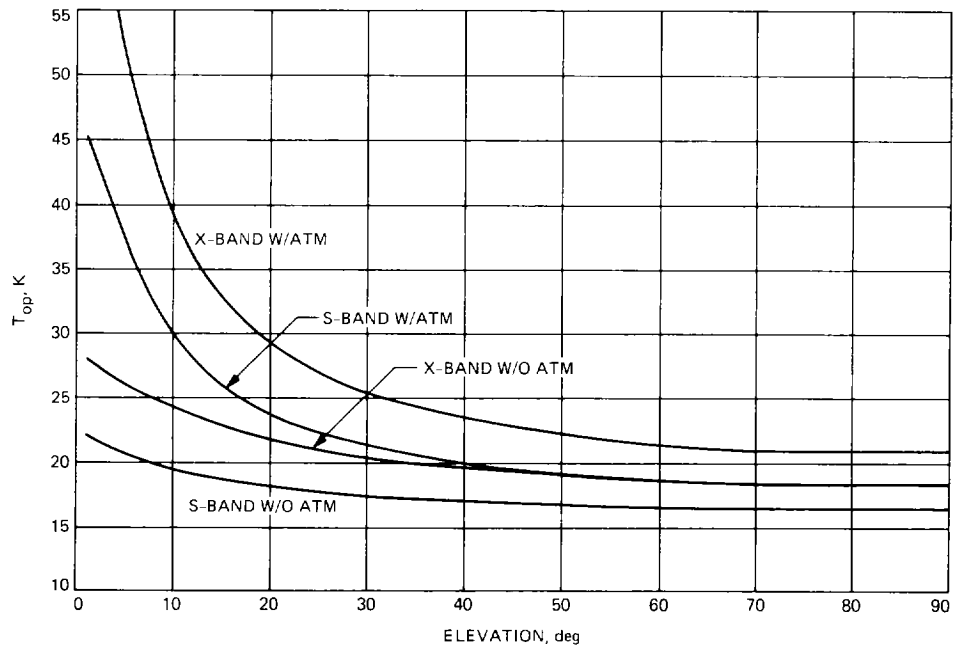
Fig. 2. S- and X-band noise temperature curve-fits, with and without atmospheric contribution.
