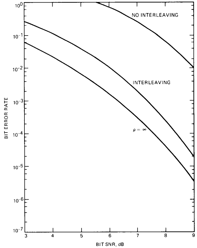
Fig. 5. Upper bound on average bit error probability versus bit energy-to-noise ratio for rate 1/2, trellis-coded QPSK; 2 states; 1/B_L T_d = 10 ; suppressed carrier.
