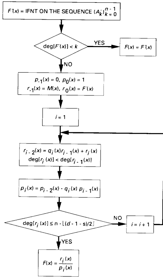
Fig. 1. Flowchart of decoding procedure to correct errors only.
