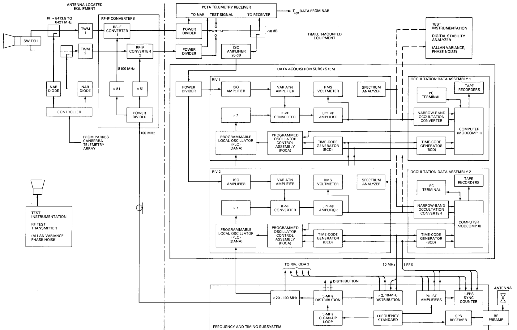
Fig. 1. Block diagram of the Parkes Radio Science System configuration.
